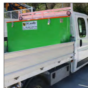
ADR exempted transportable tanks in painted carbon steel. Transportable carbon steel tank for diesel with ADR exemption DIESELBOX & TOOLS
